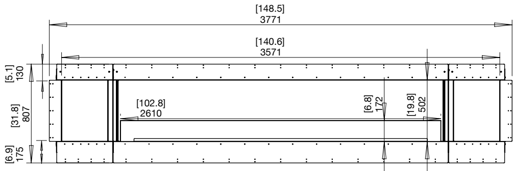
ESF.FX.140SS.BX2 (Left & Right Decorative Box)
